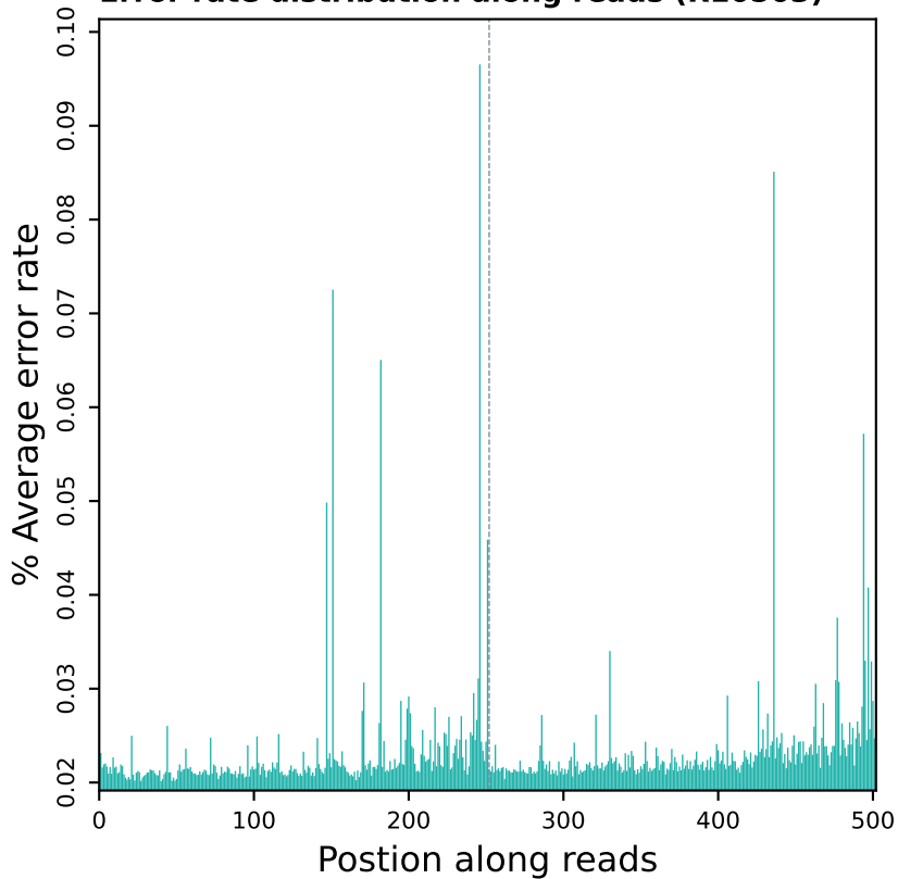
Error rate distribution along reads (R10503)
